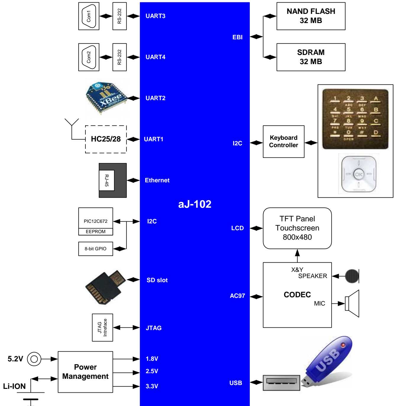
Figure 1. Block Diagram of aJ-102DEK
